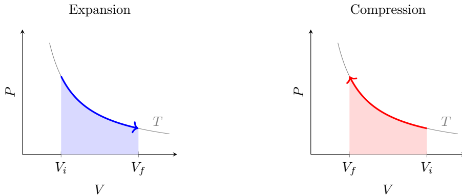
Figure 2: Isothermal processes of an ideal gas. The shaded area under the isotherm is |W| . Left: expansion, W < 0 and heat flows in. Right: compression, W > 0 and heat flows out.
